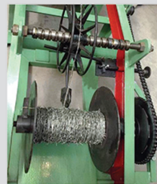
Barbed Wire Machine
