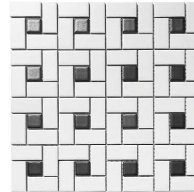
KQD-1005/810 chip size: 23x48/23x23mm sheet size: 300x300mm
